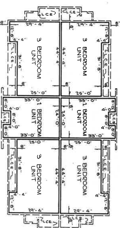
TYPICAL BUILDING ABOVE IS THE APPROXIMATE REPRESENTATION OF THE FOLLOWING UNITS: 21A-F, 24A-F, 25A-F, 26A-F, 27A-F, 28A-F.
